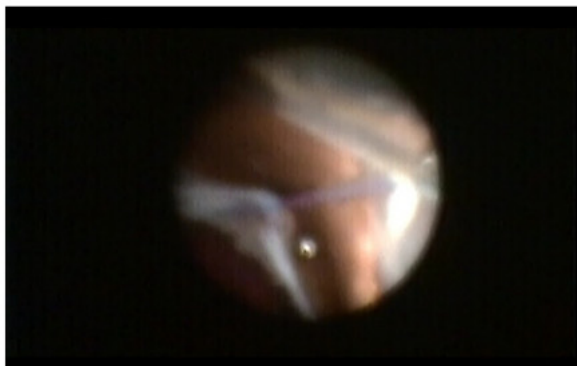
Fig. 8 – Verification of intraocular lens (IOL) position and capsular support. The endoscopic view shows a patient with a subluxated IOL undergoing repositioning of the implant. The patient has a compromised posterior capsule, and a sulcus placed IOL was the desired placement. However, in the endoscopic view, the inferior haptic is identified to be posterior to the anterior capsule, and therefore in the compromised capsular bag, predisposing to further subluxation. The haptic was retrieved and placed in the sulcus, anterior to the capsule.
