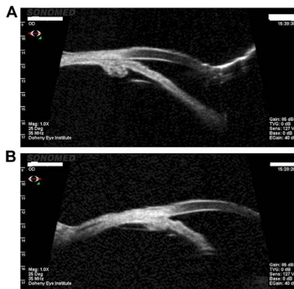
Fig. 2 – Endoscopic cilioplasty for plateau iris syndrome. A: The ultrasound biomicroscopy image shows the preoperative appearance of severe plateau iris with appositional angle closure caused by large and anteriorly rotated ciliary processes pushing the peripheral iris anteriorly. B: Following ECPL and lens extraction, the angle is wide open and the ciliary processes are flattened and shrunken.
